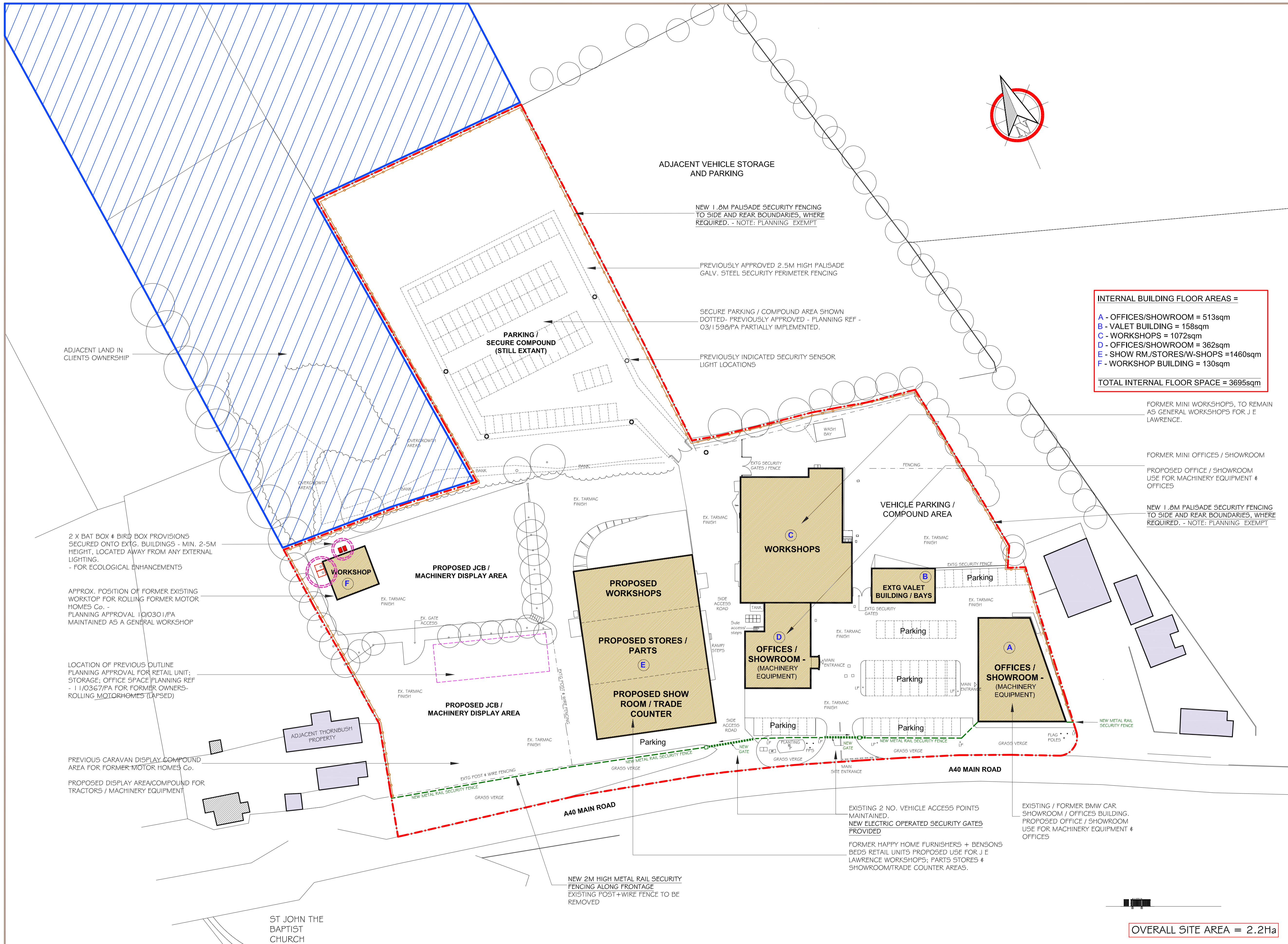
OVERALL SITE LAYOUT - 1:500
