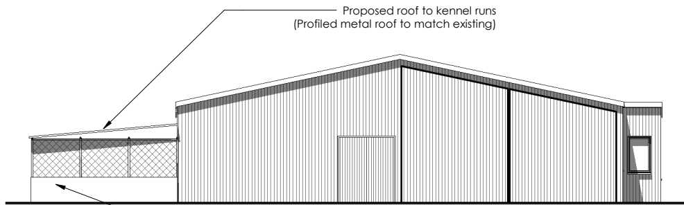
South 1 : 100
